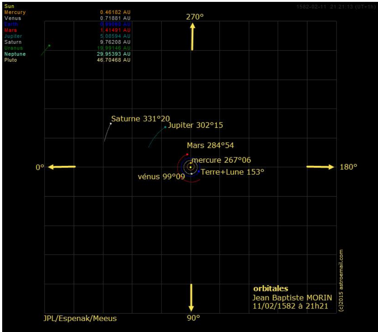
JB Morin orbital from Sun to Saturn
